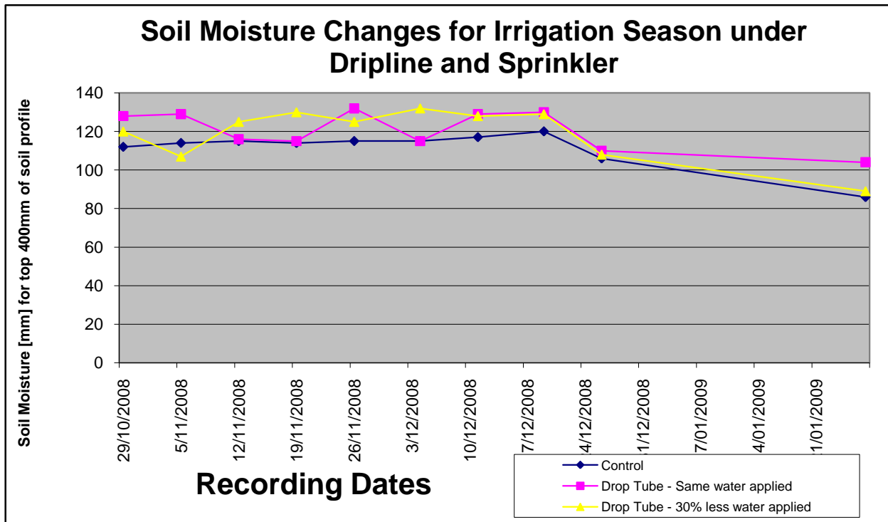
Graph 3: Soil moisture changes over the irrigation season
